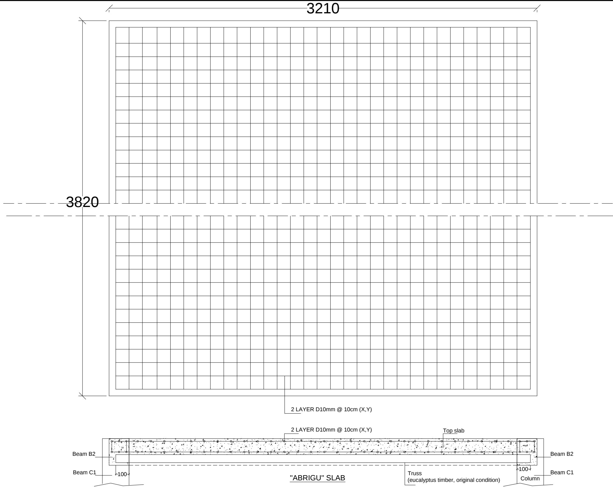
"ABRIGU" TOP SLAB STRUCTURE DETAILS 1:200
