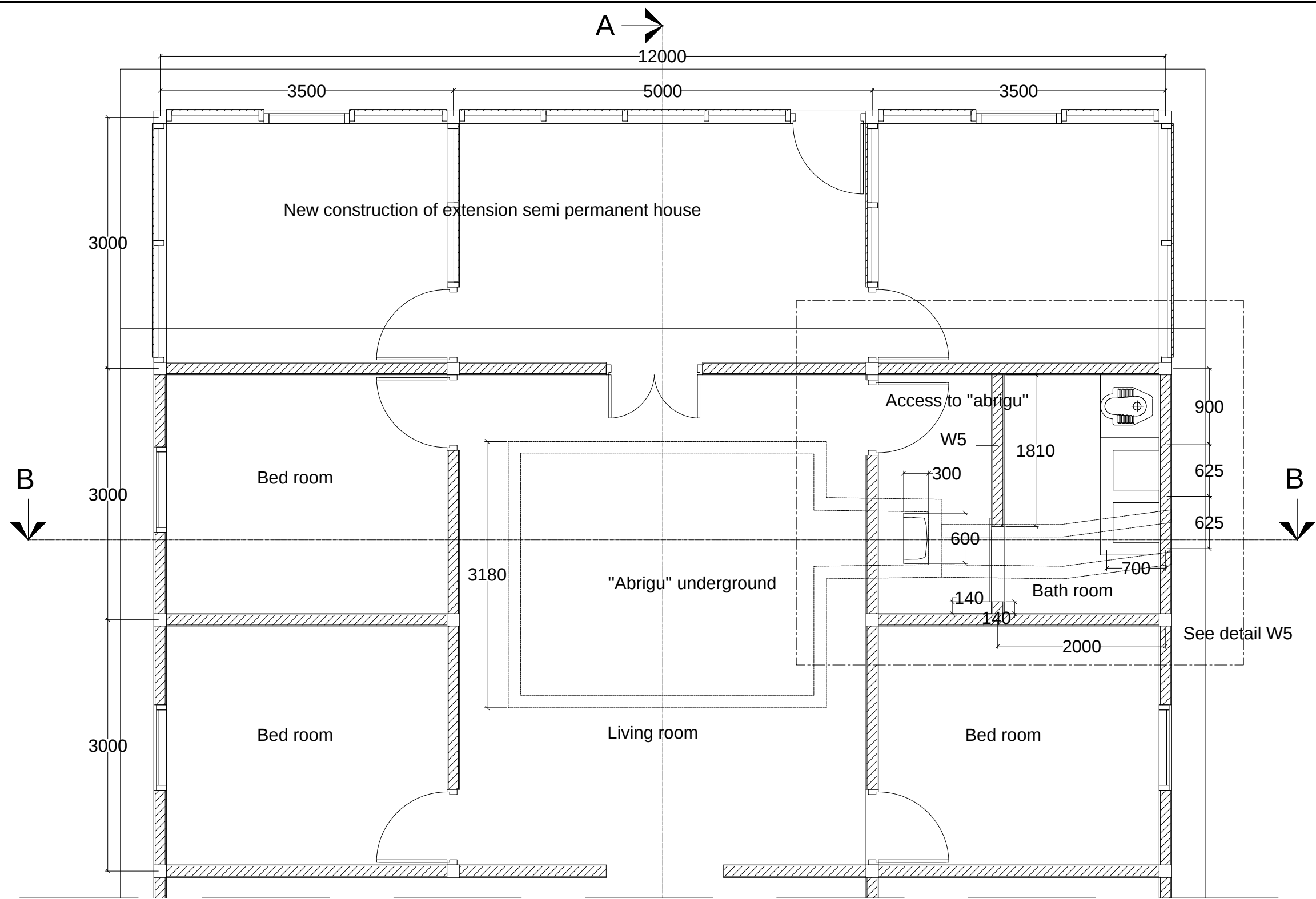
"ABRIGU" EXISTING LOCATION PLAN LAY OUT 1:200
