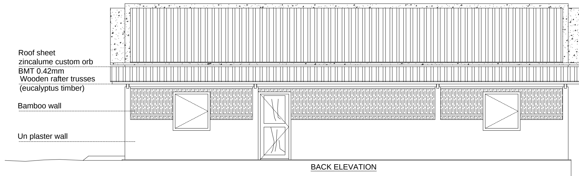
EXTENSION HOUSE PLAN 1:200
