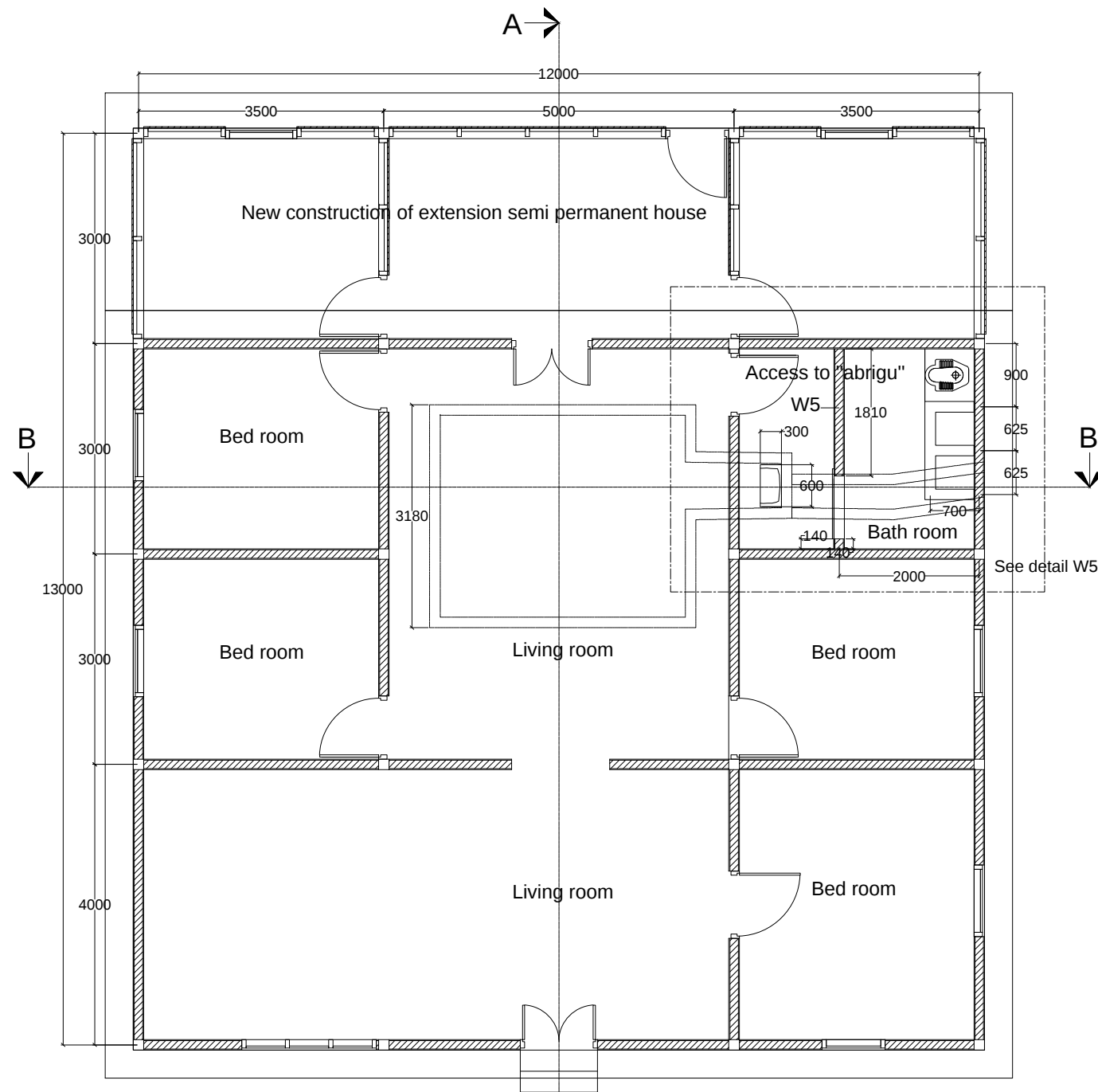
EXISTING PLAN 1:200
