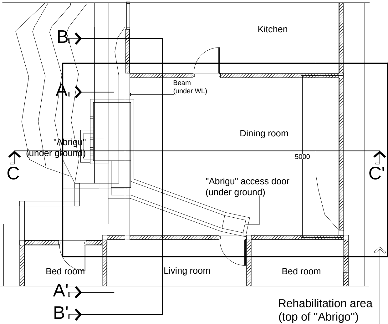
REHABILITATION PLAN
