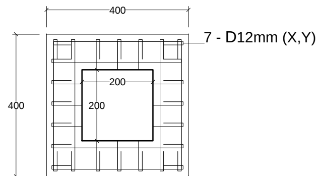
FOOT PLATE & COLUMN
