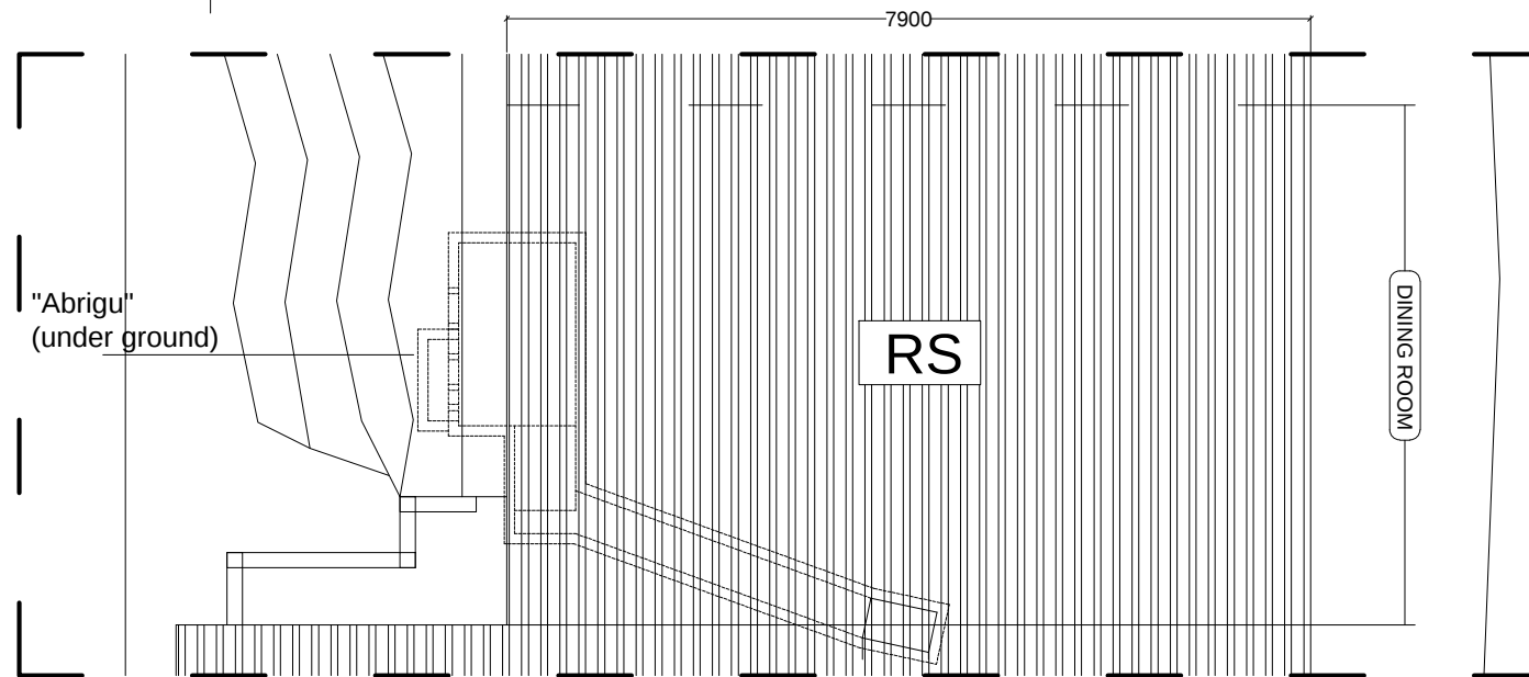
ROOF SHEETS
