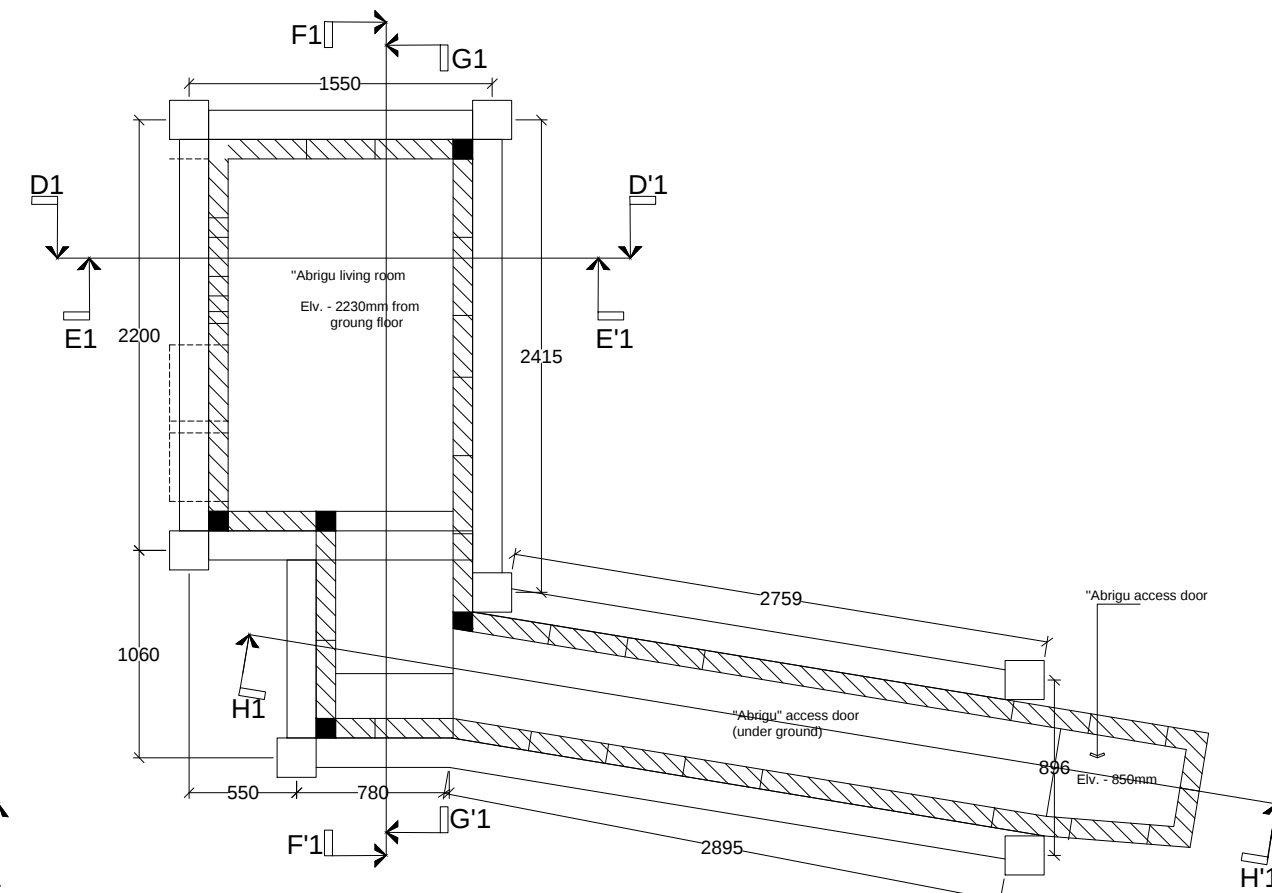
"ABRIGU" TOP BEAM PLAN
