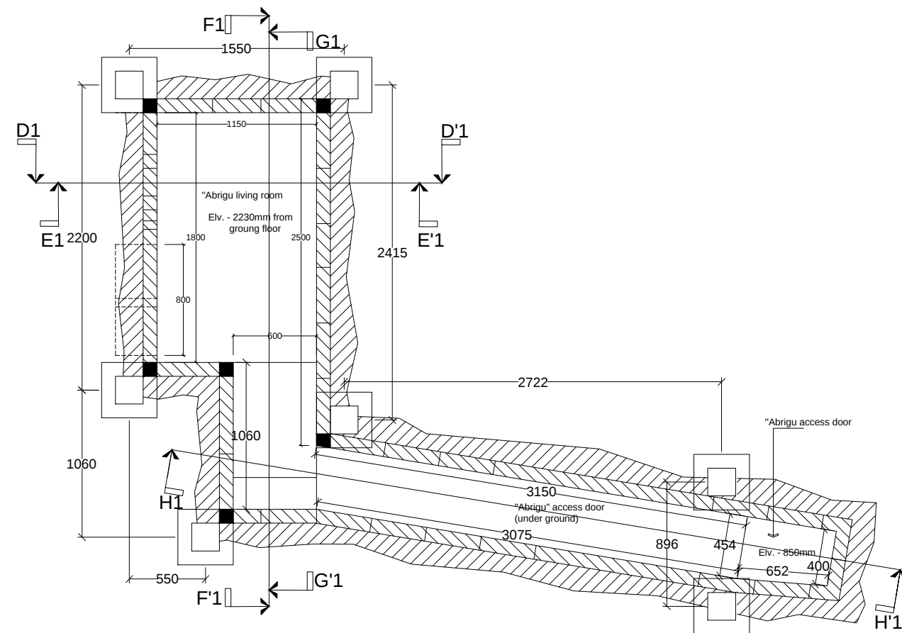
"ABRIGU" FOOT PLATE AND COLUMN PLAN
