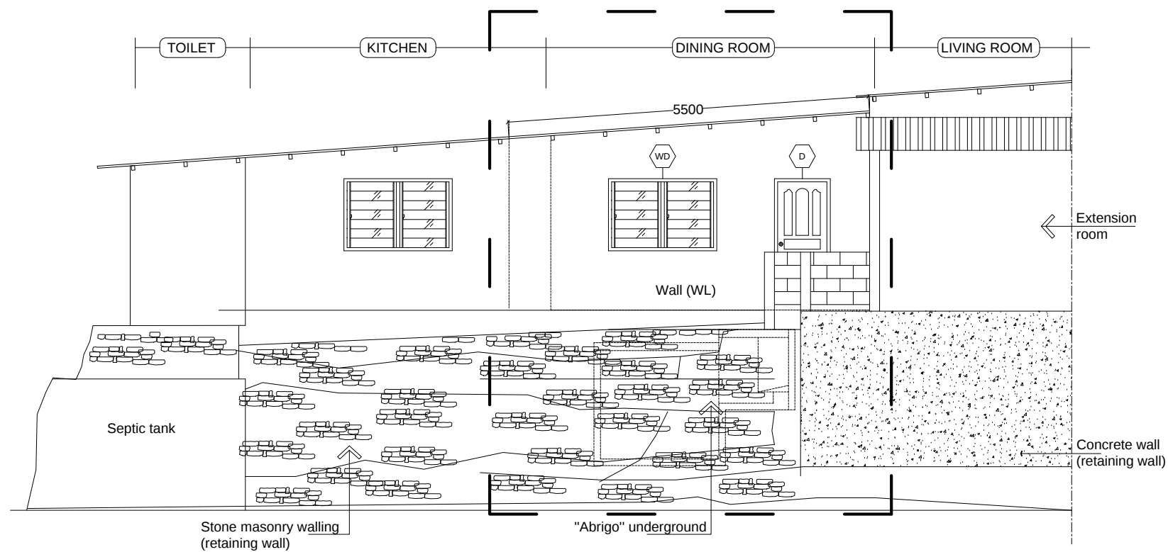
SIDE VIEW
