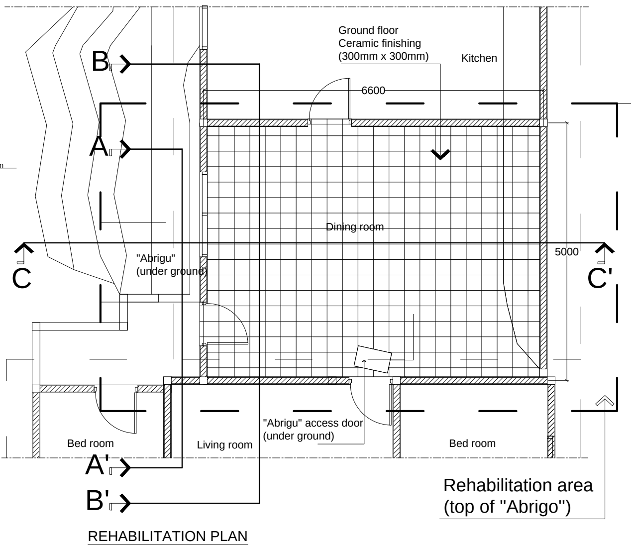
FLOOR PLAN (CERAMIC) 1:1500
