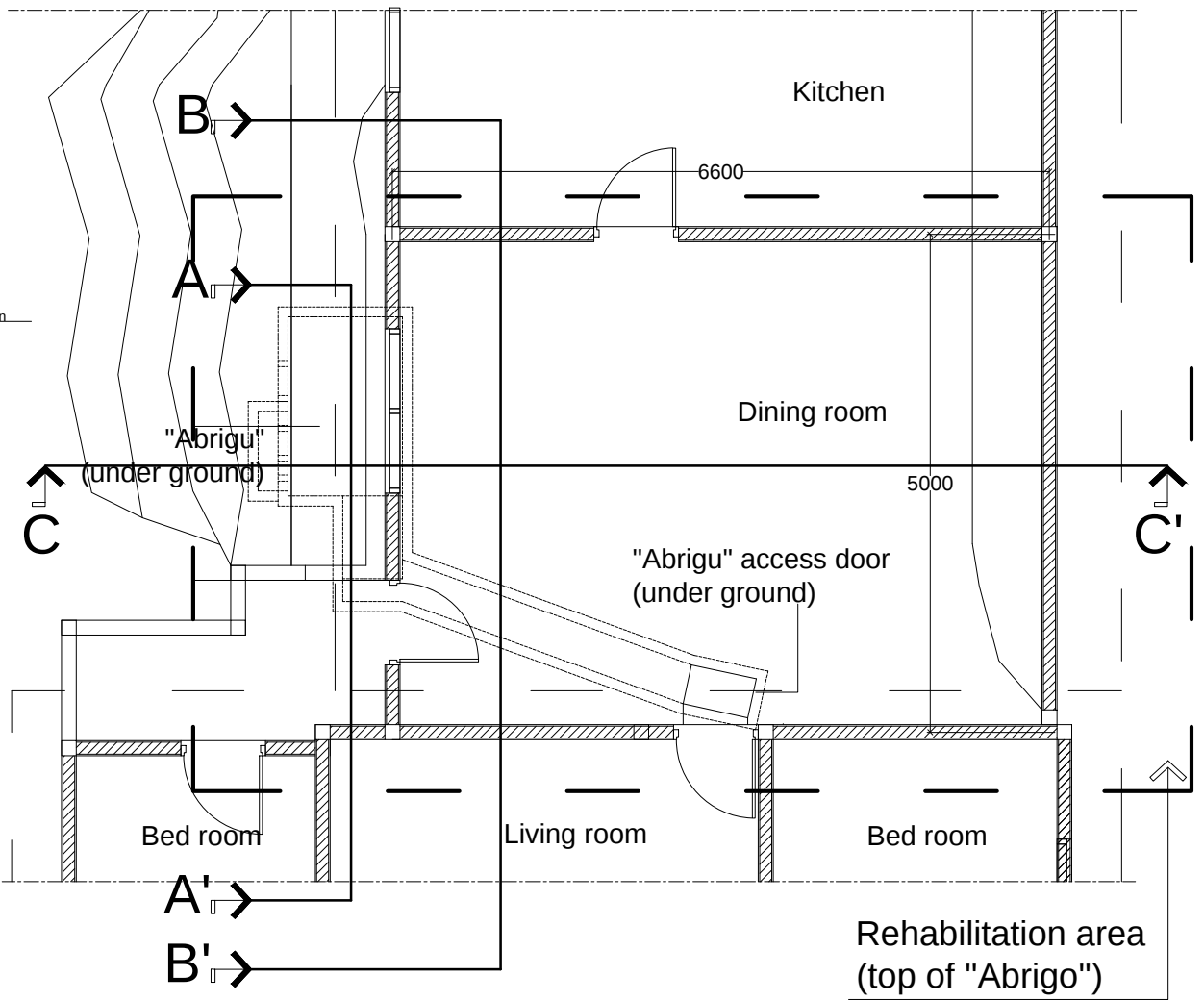
REHABILITATION PLAN
