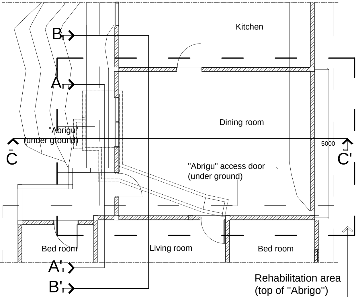
REHABILITATION PLAN
