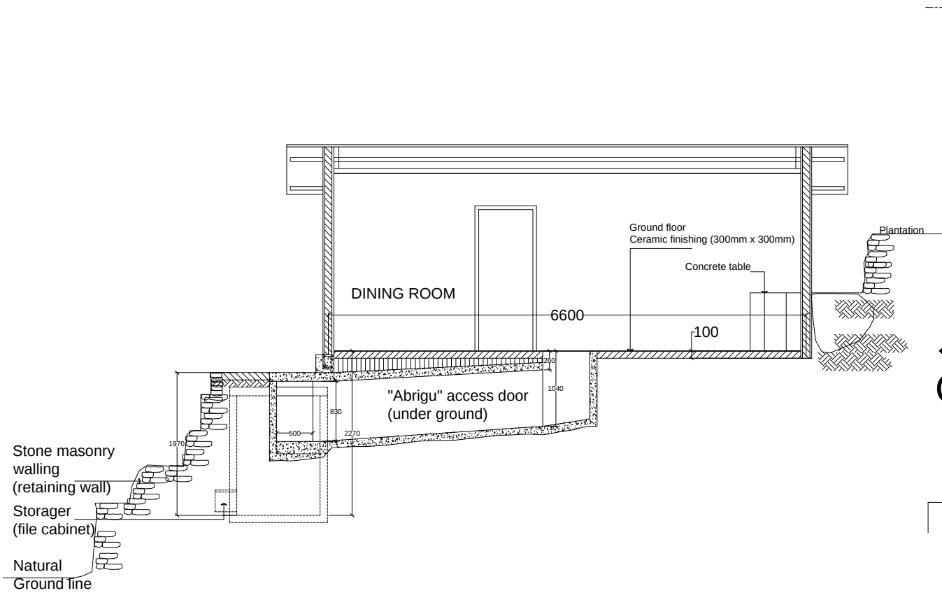
SECTION H-H
