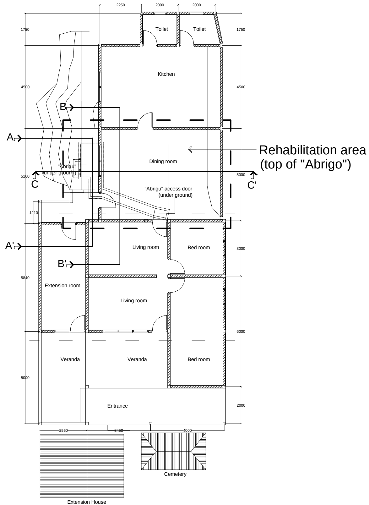
EXISTING PLAN 1:3000
