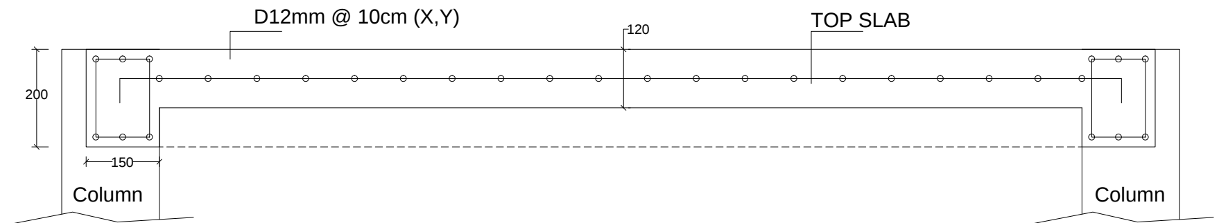
"ABRIGU" TOP SLAB AND BEAM
