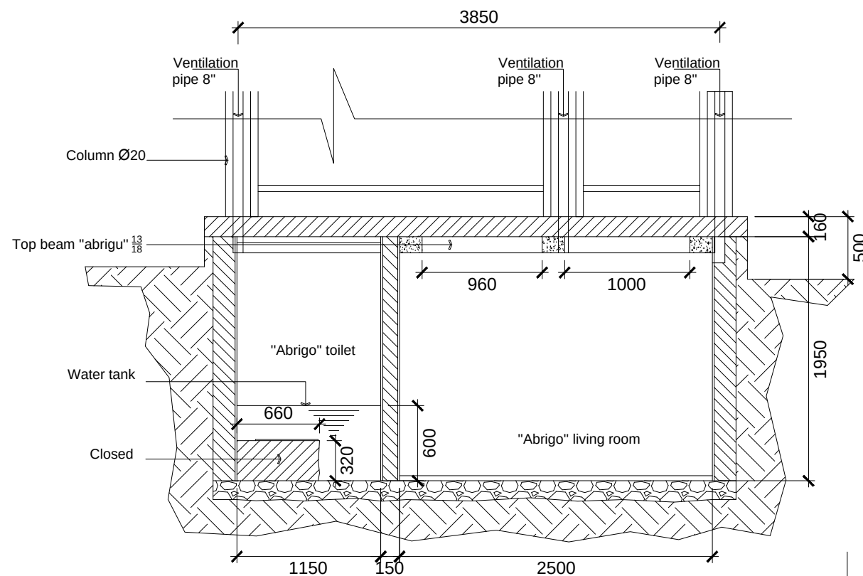
SECTION C-C
