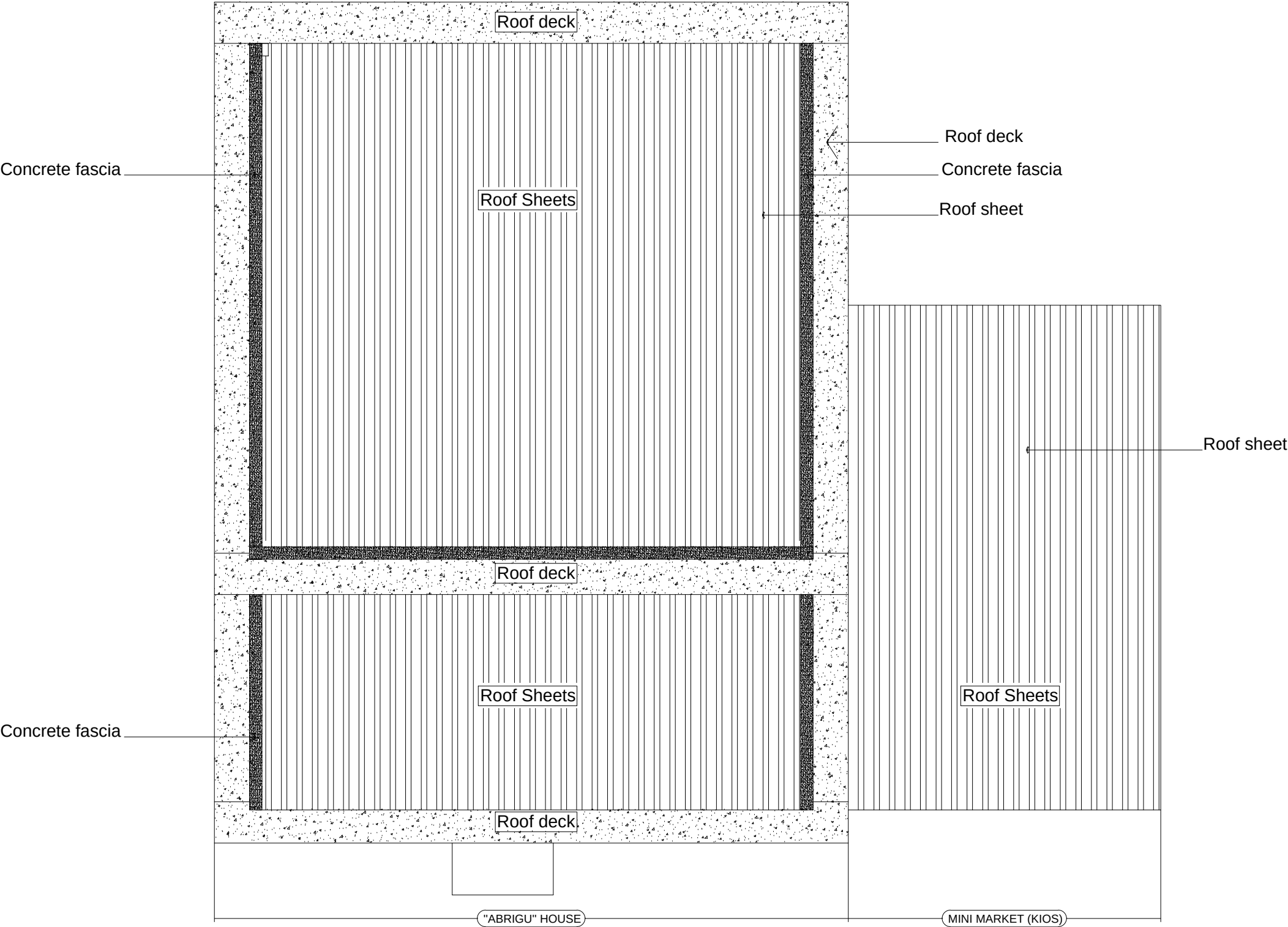
TOP ROOF
