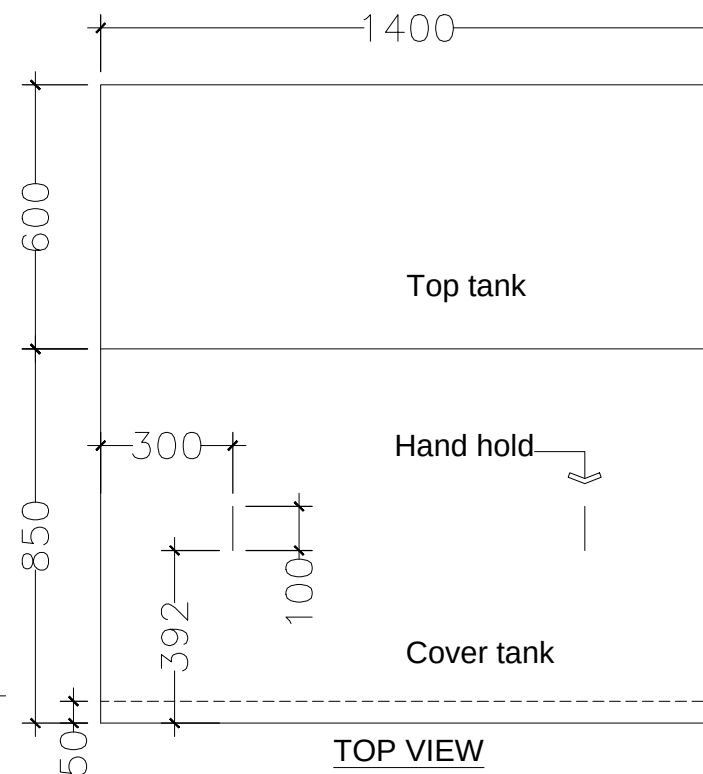
WATER TANK COVER DETAILS
