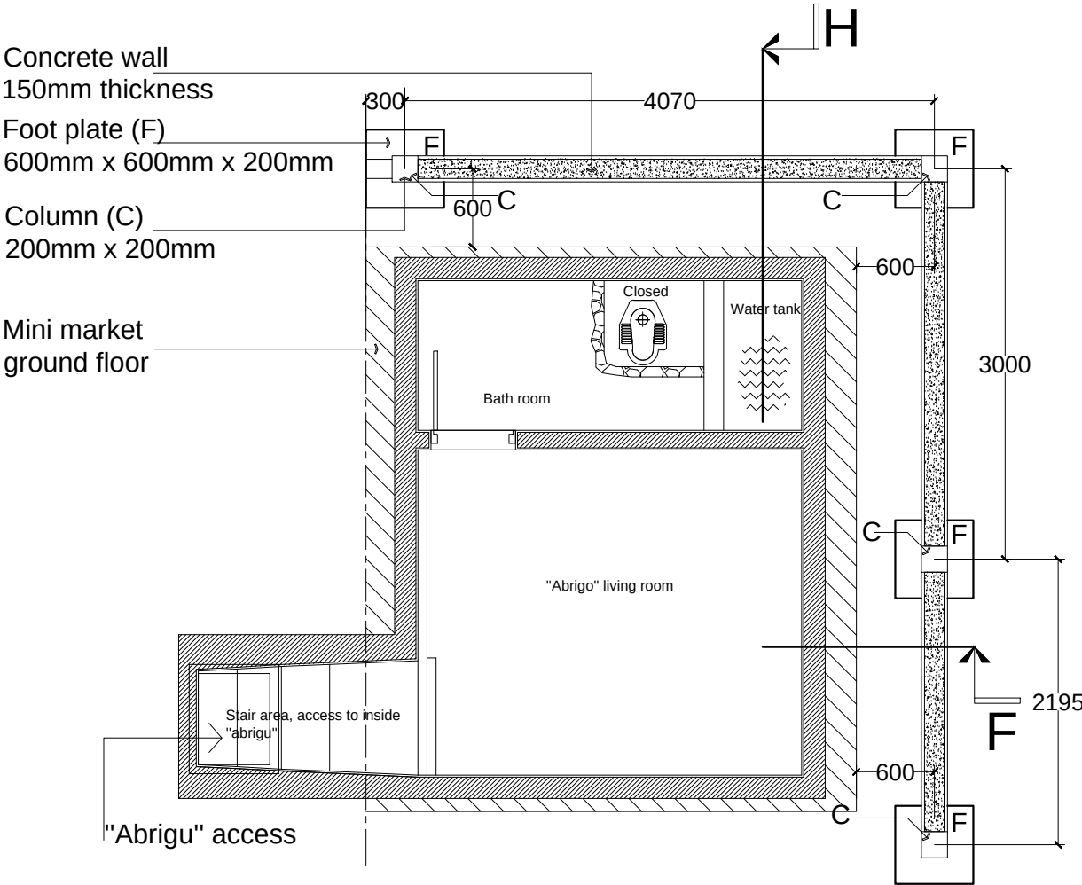
"ABRIGU" RETAINING WALL PLAN 1:1000
