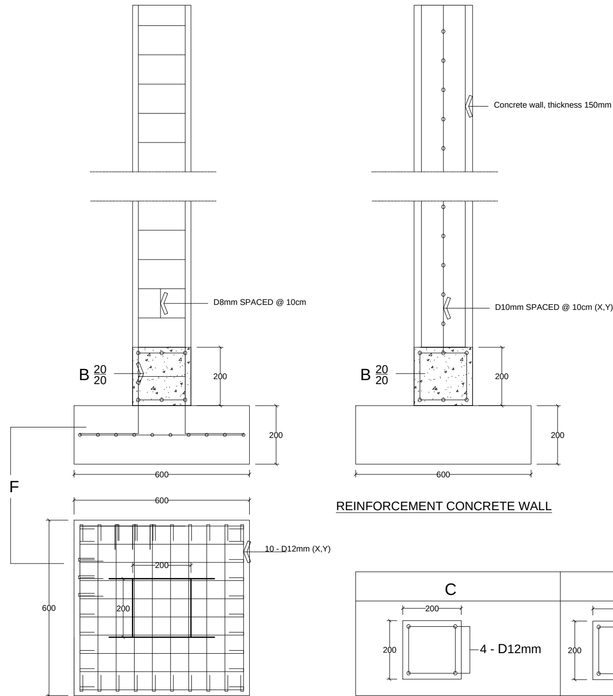
FOOT PLATE & COLUMN
