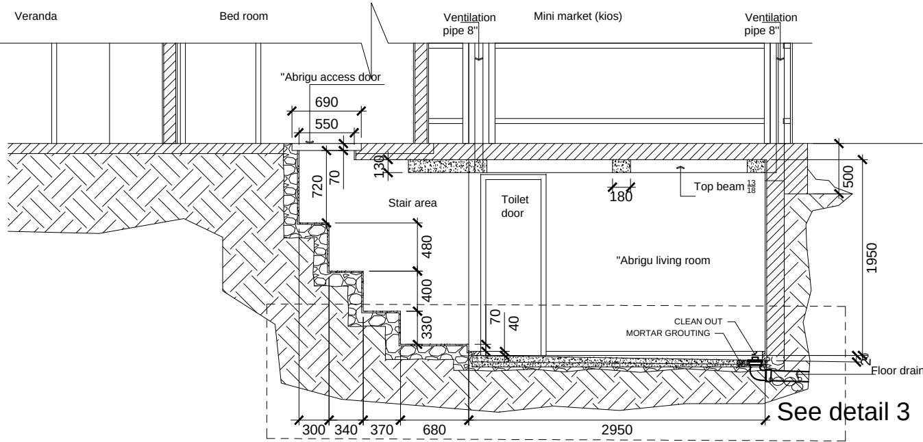
LEAN CONCRETE "ABRIGU" FLOOR 1:1000
