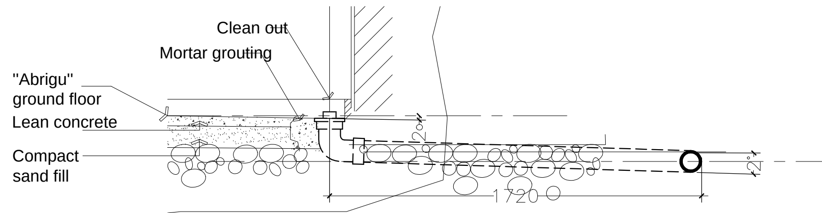
"ABRIGU" FLOOR DRAIN DETAILS
