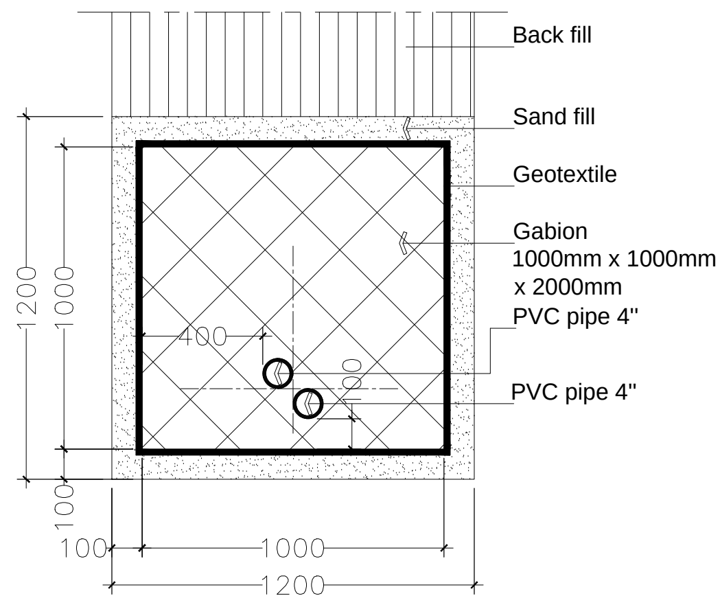
GABION INSTALLATION AND DETAILS (DETAIL 4)
