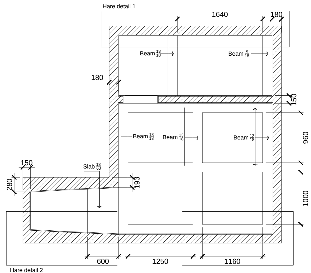
EXISTING TOP BEAM
