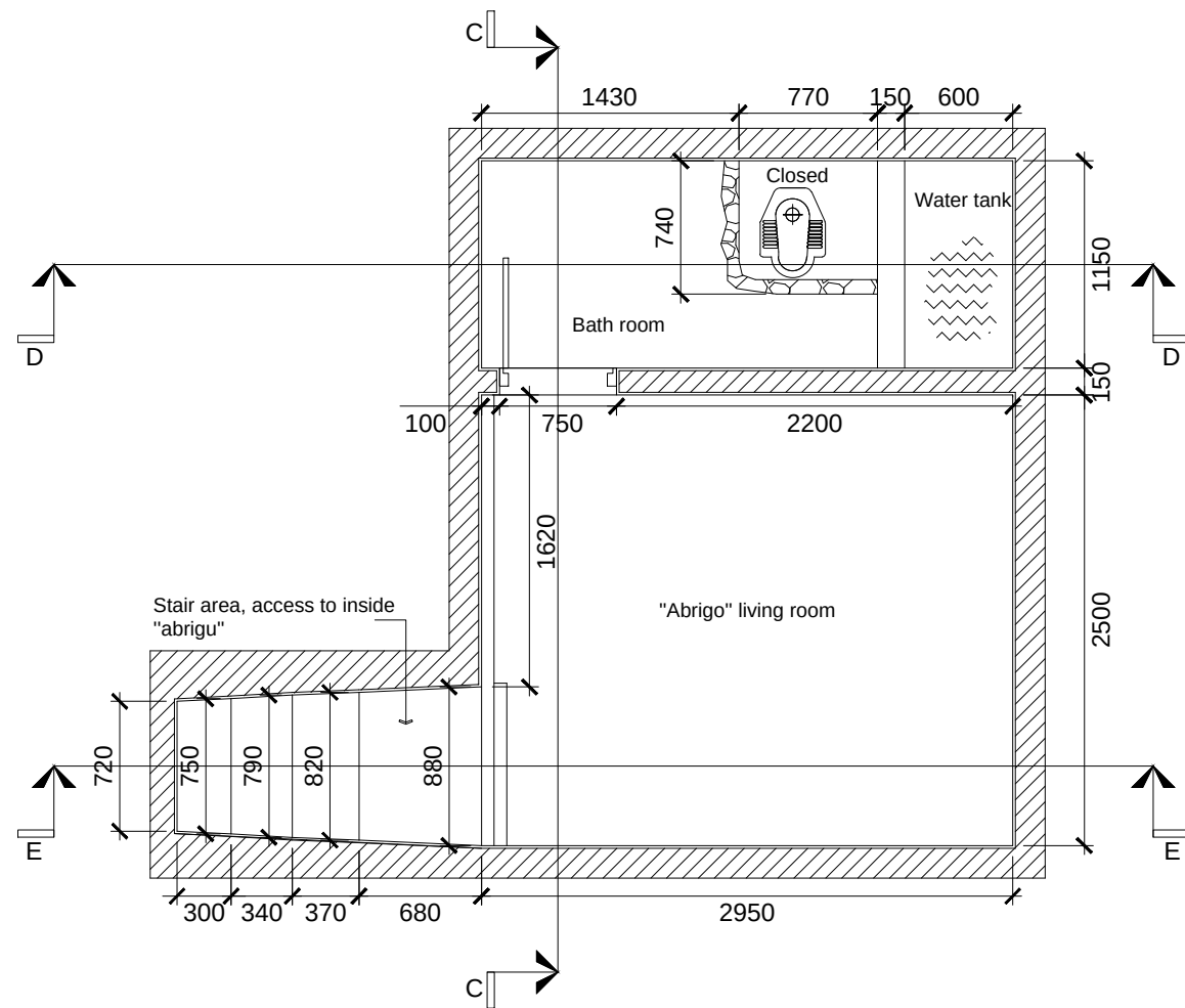
"ABRIGU" EXISTING PLAN
