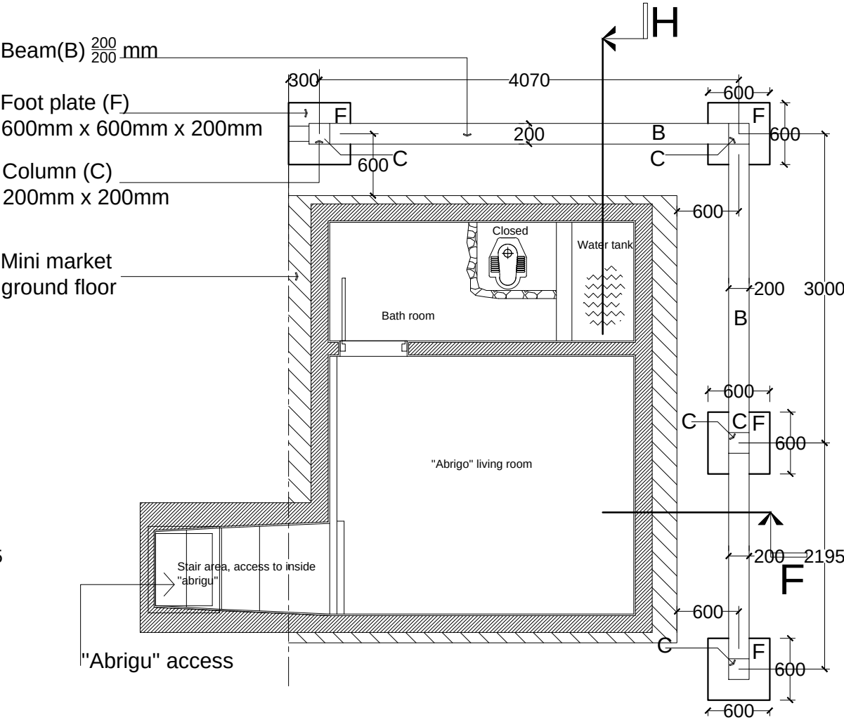
FOOT PLATE, COLUMN, BEAM PLAN 1:1000
